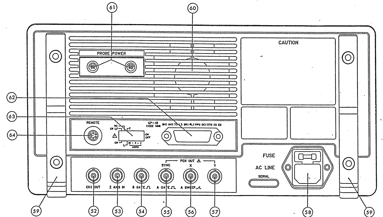
Figure 4-2. Rear Panel
