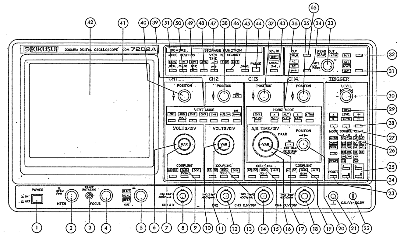
Figure 4.1. Front Panel
